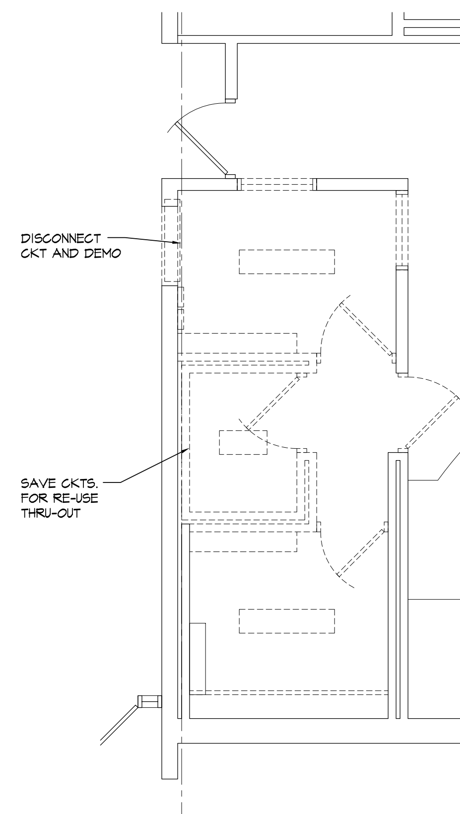
EXISTING ELECTRICAL PLAN- DEMO.
