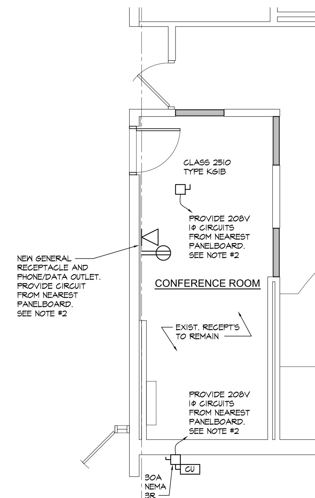
ELECTRICAL POWER PLAN
