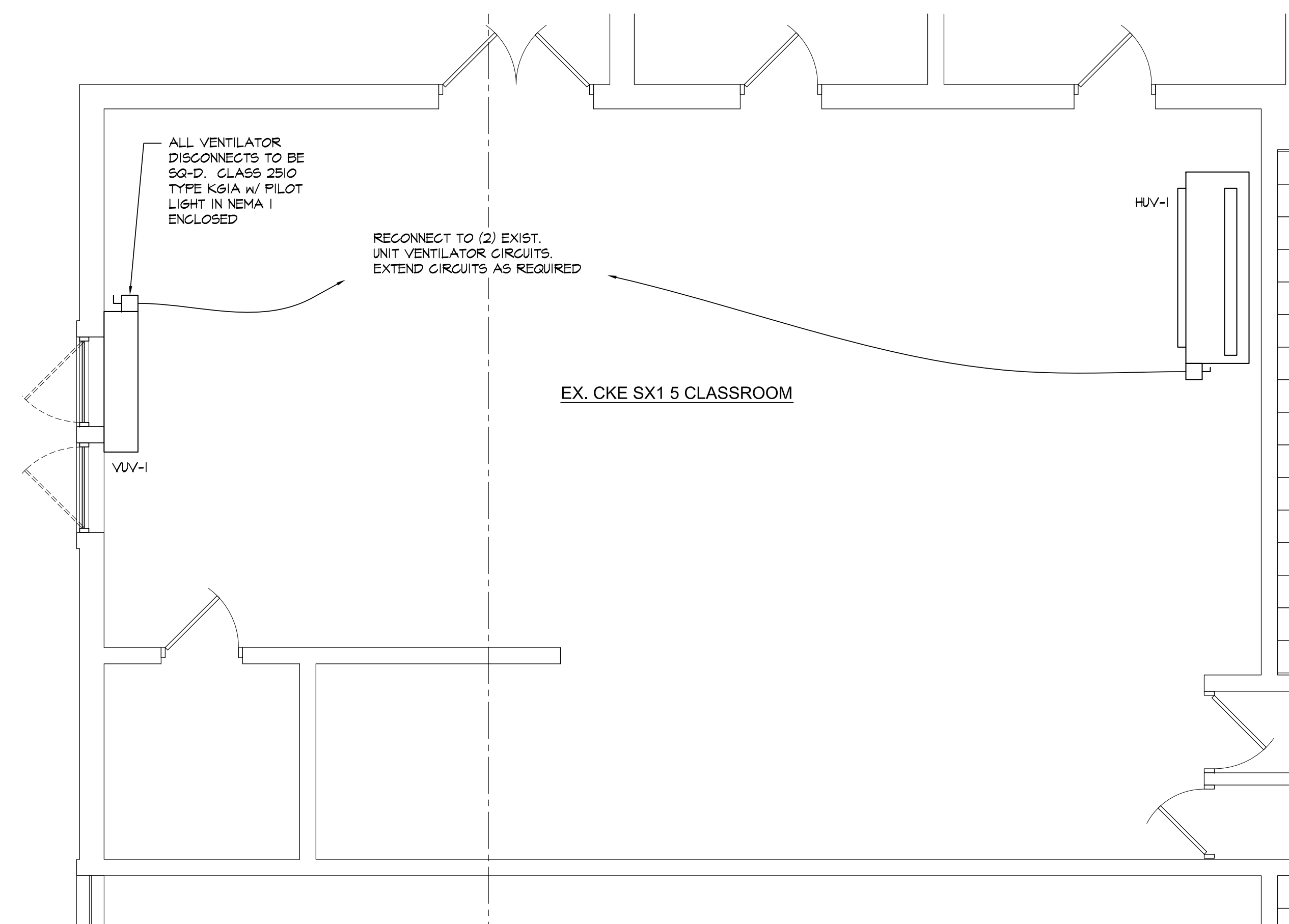
PROPOSED FLOOR PLAN
